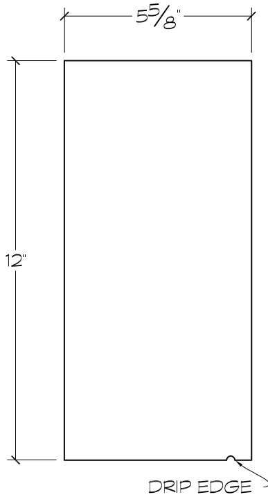
CROSS SECTION
